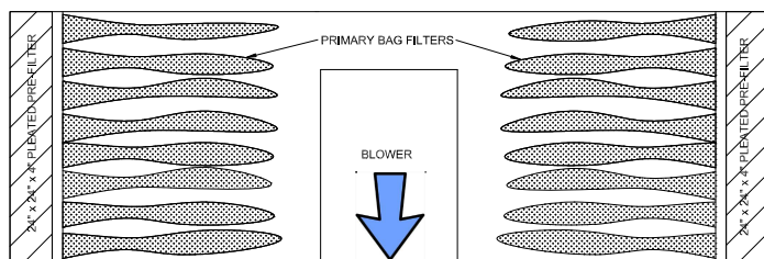
TOP VIEW : CUT-AWAY
