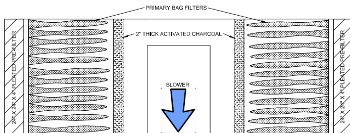
TOP VIEW : CUT-AWAY
